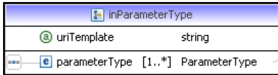
Figure 3. Specification for inParameterType .
